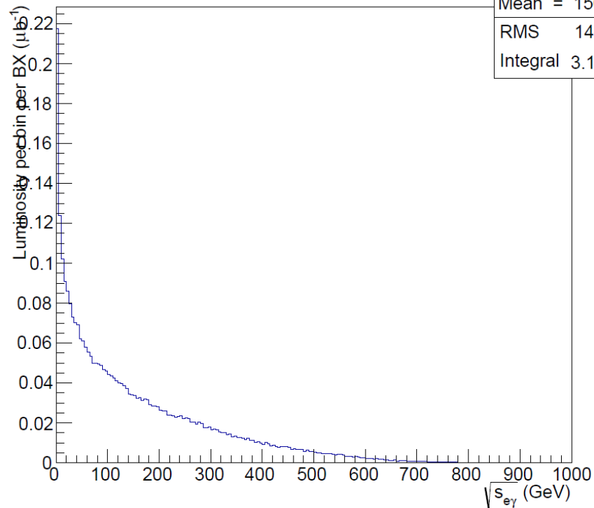
e^- \gamma Luminosity Spectrum ILC1000
